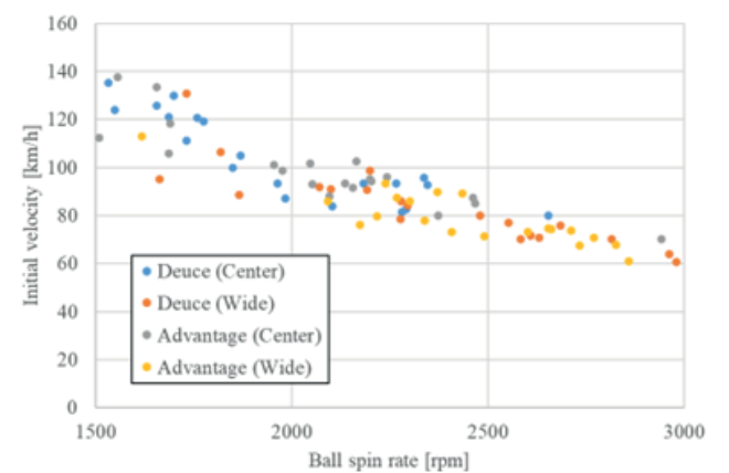
Figure 9. Relationship between ball spin rate and initial velocity
